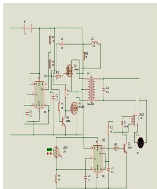
Fig. 2. Circuit Diagram of Single Phase Series Resonant Inverter
