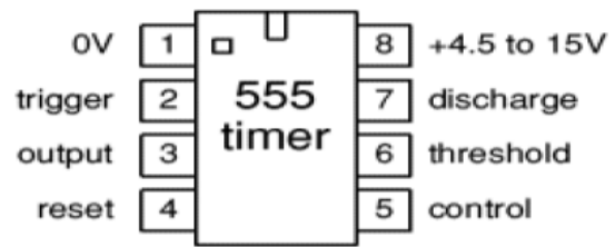
Fig: 6. Showing NE555 Timer
