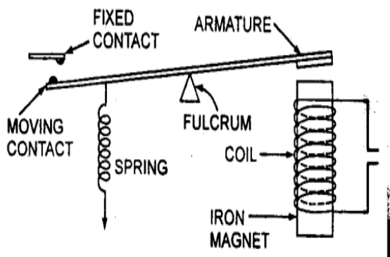
Fig: 6. Basic Diagram Showing the Operating Principle of a Relay
